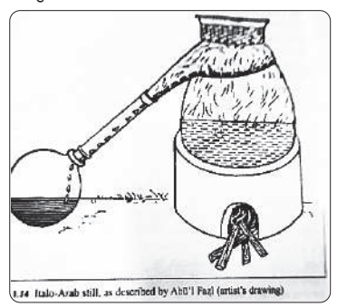
Fig. 1.4. Indo-Arab still, as described by Abū'l Fajr (artist's drawing)
